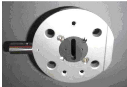
Signet's Ground Electrode with Replaceable Graphite Ion Slot
