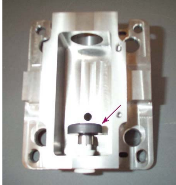
Signet Products PN 1110 Kit in a GSD Arc Chamber
