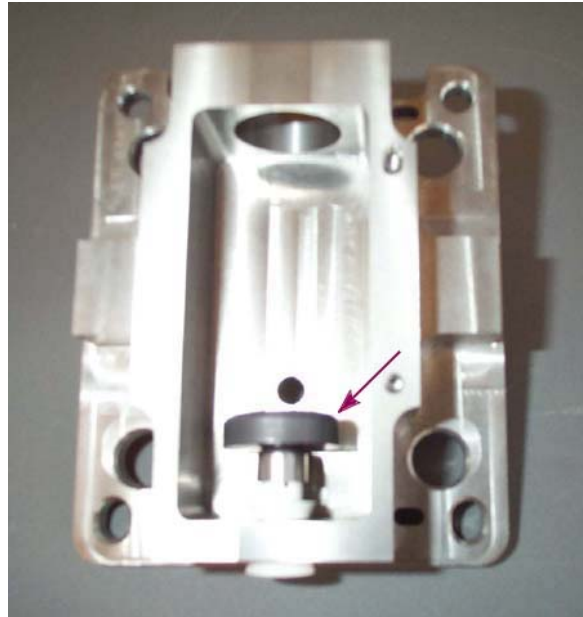
Signet 40-2760 in a GSD Arc Chamber
