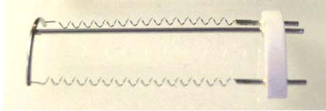
Signet Part Number 30-0095 Replacement Dual tungsten Filaments
