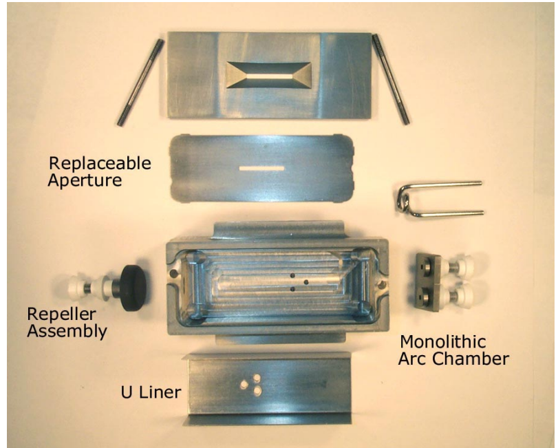
Conversion Kit Signet Part Number 1042-1
