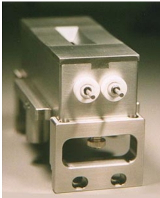
Assembled Bernas Arc Chamber
